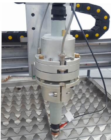
Electronic Torch Breakaway
